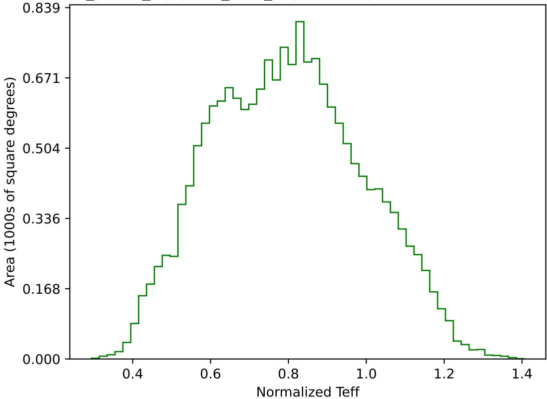
roll_pause_mjdp180_v3.4_10yrs WFD g band: Normalized Teff
