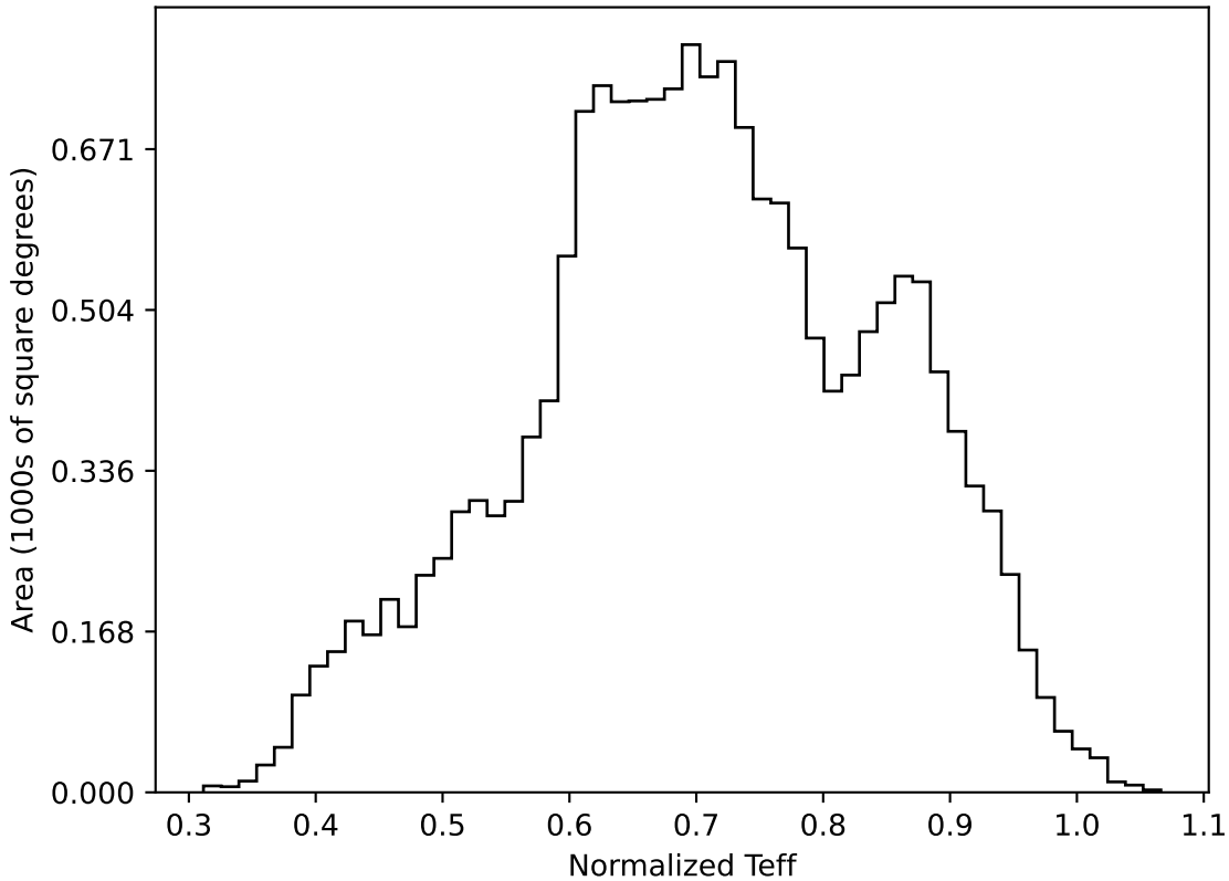
roll_pause_mjdp180_v3.4_10yrs WFD all bands: Normalized Teff
