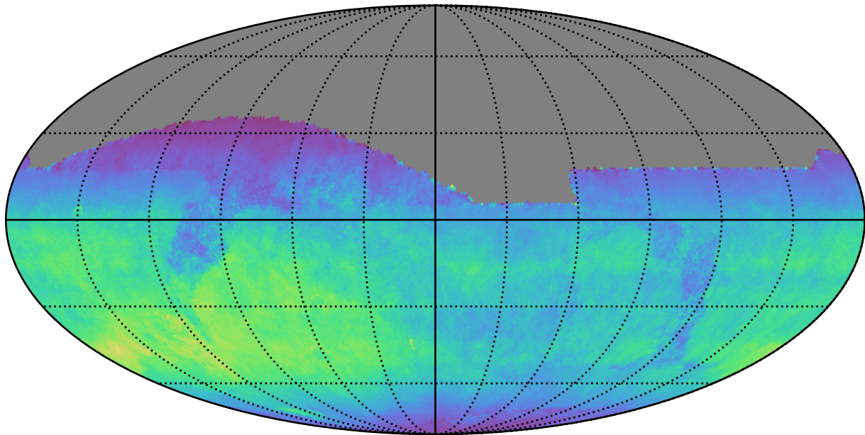
roll_pause_mjdp180_v3.4_10yrs All sky z band: Normalized Teff
