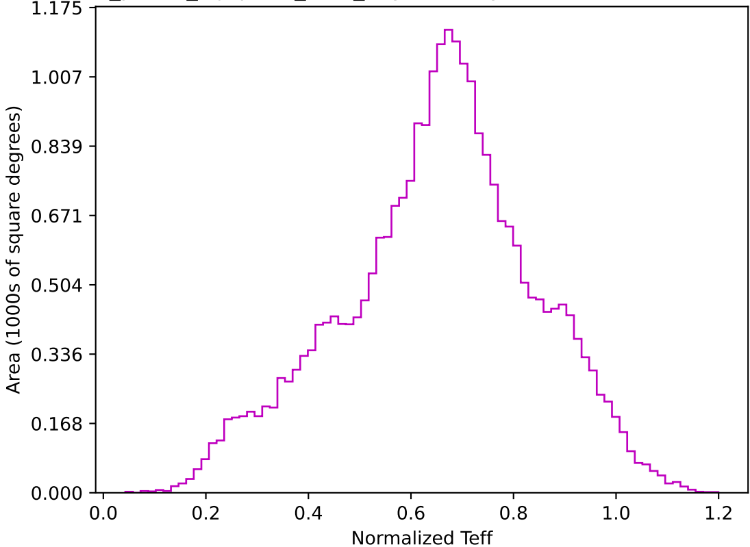
roll_pause_mjdp180_v3.4_10yrs All sky z band: Normalized Teff
