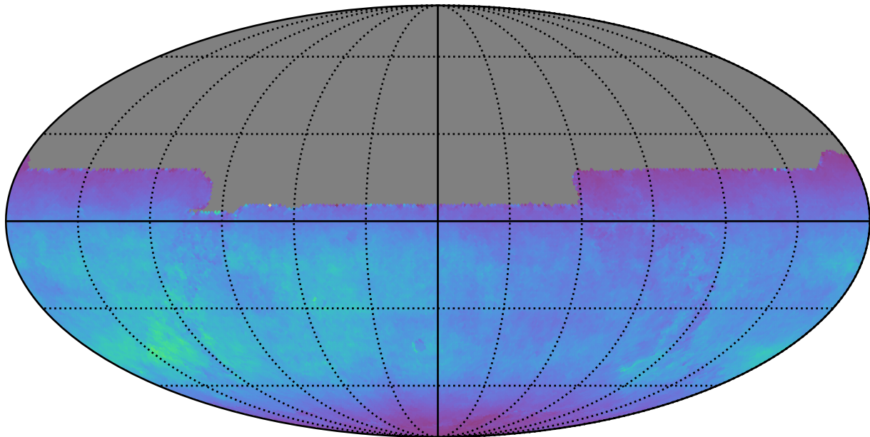
roll_pause_mjdp180_v3.4_10yrs All sky y band: Normalized Teff
