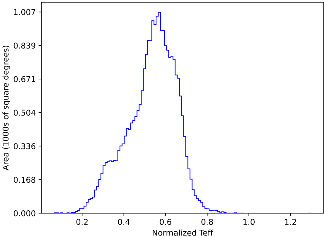
roll_pause_mjdp180_v3.4_10yrs All sky y band: Normalized Teff
