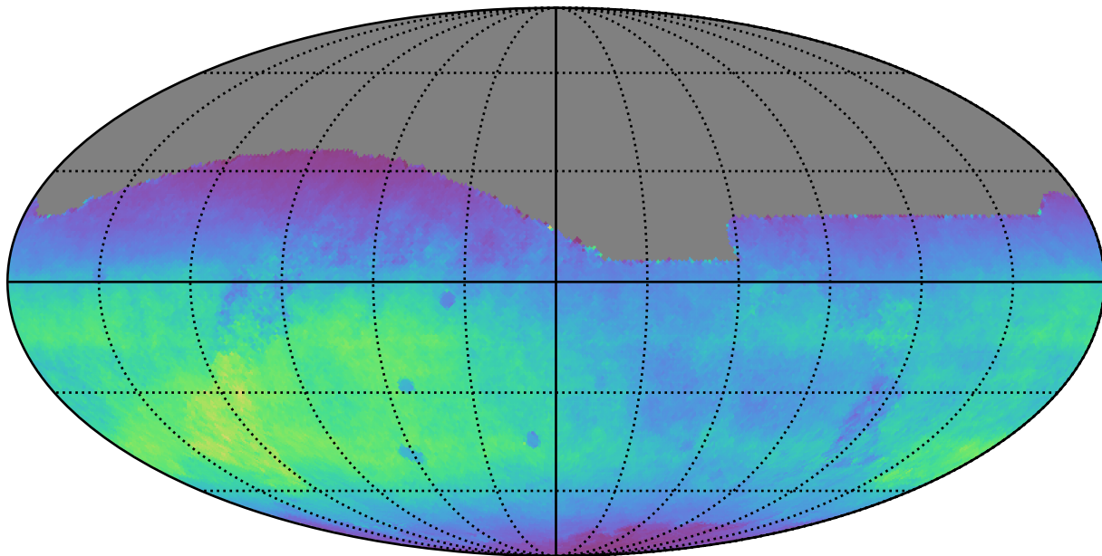
roll_pause_mjdp180_v3.4_10yrs All sky r band: Normalized Teff
