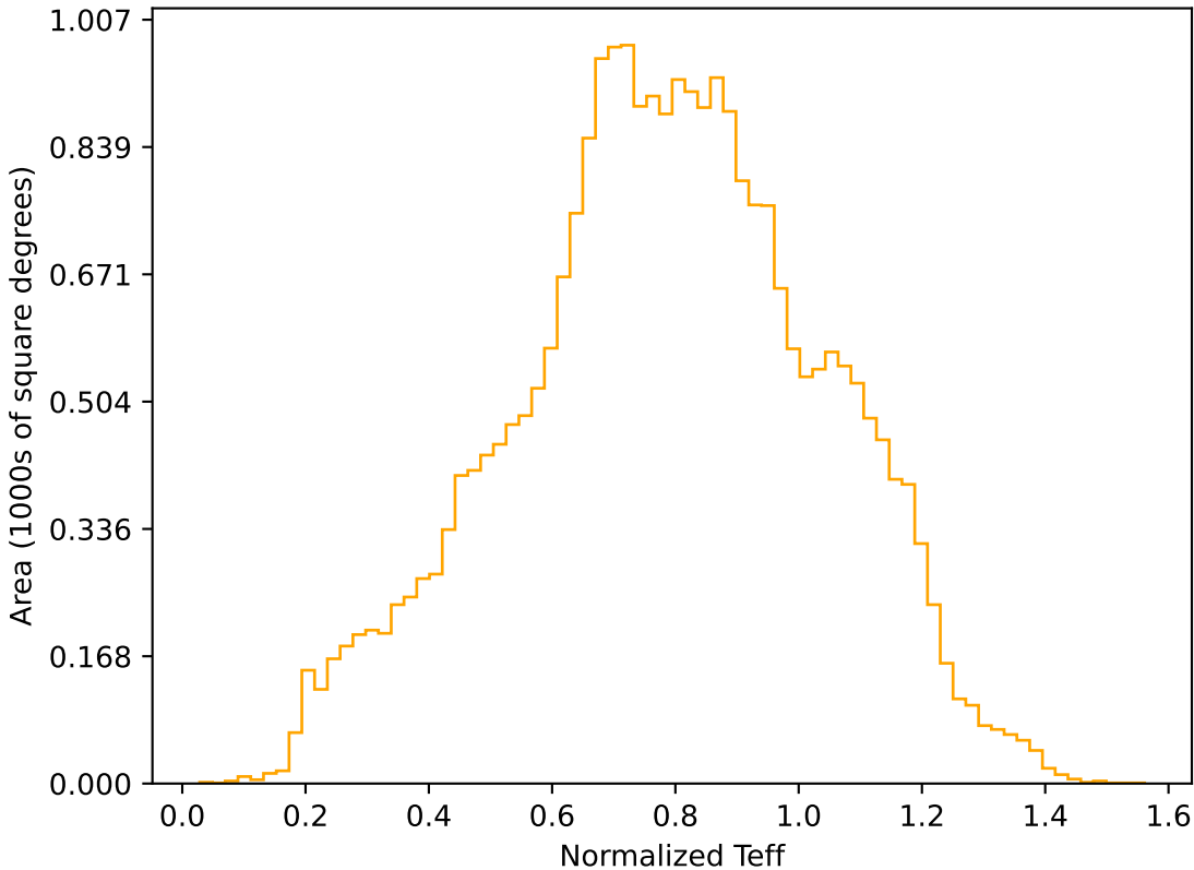
roll_pause_mjdp180_v3.4_10yrs All sky r band: Normalized Teff
