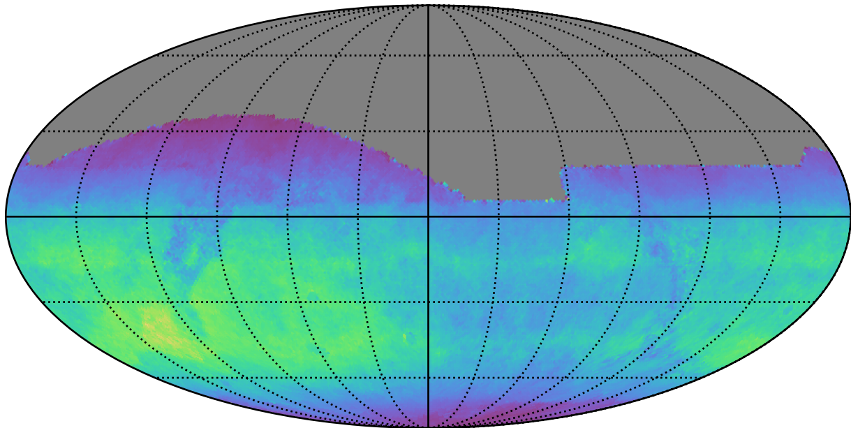
roll_pause_mjdp180_v3.4_10yrs All sky i band: Normalized Teff
