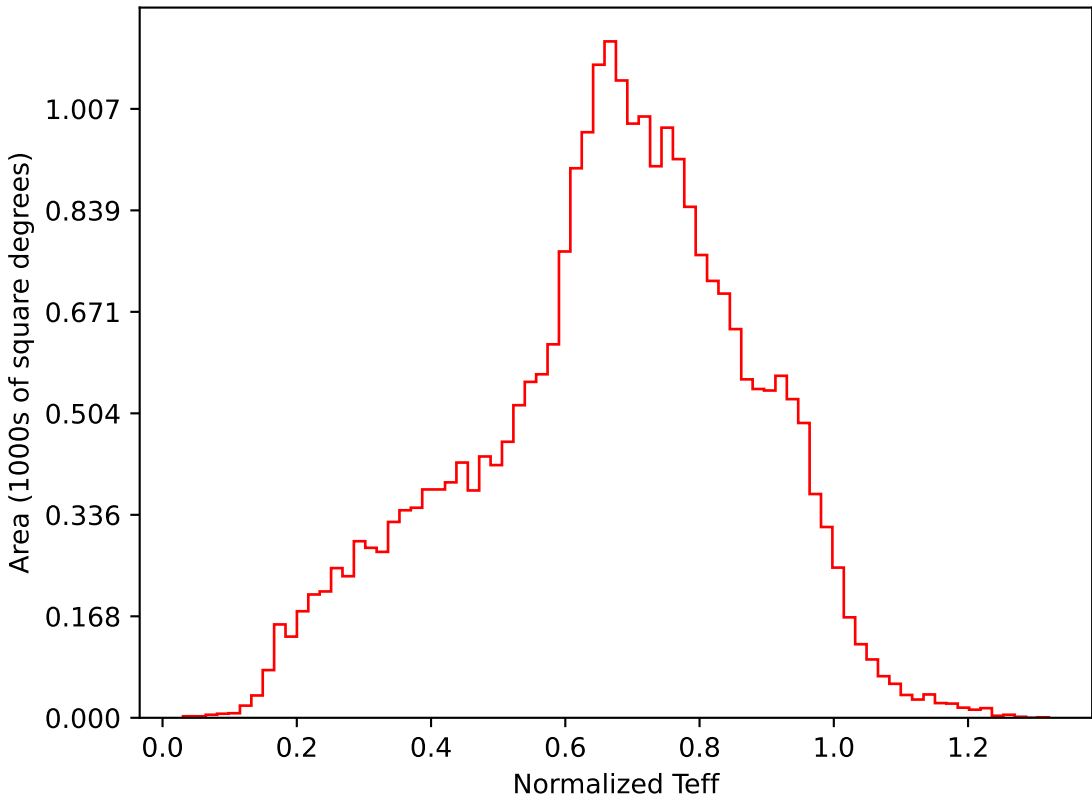
roll_pause_mjdp180_v3.4_10yrs All sky i band: Normalized Teff
