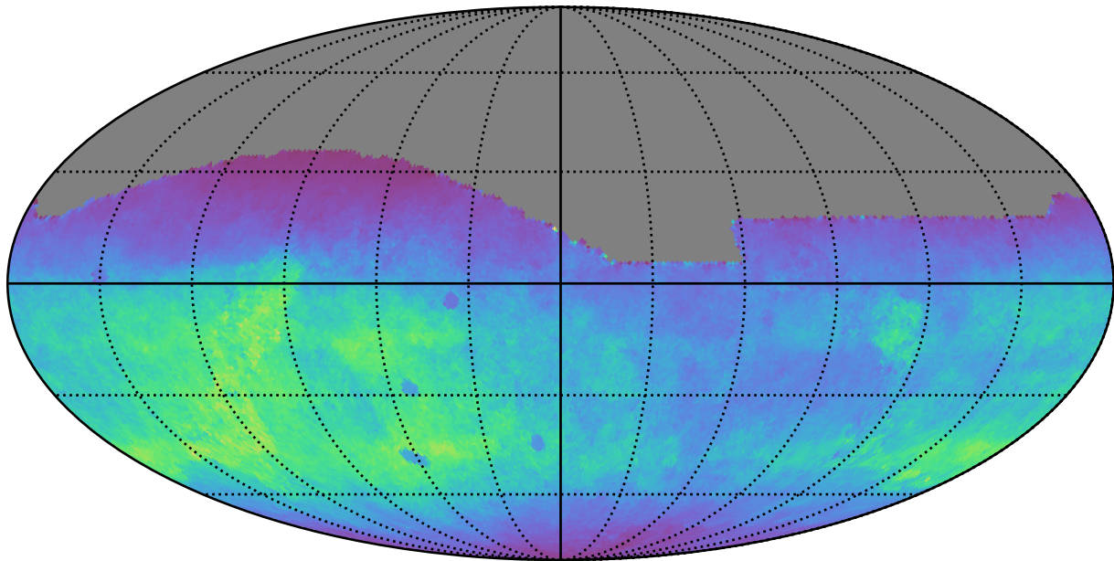
roll_pause_mjdp180_v3.4_10yrs All sky g band: Normalized Teff
