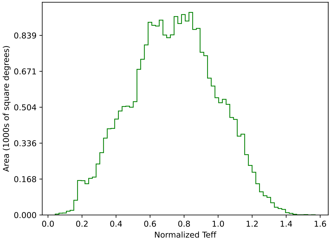
roll_pause_mjdp180_v3.4_10yrs All sky g band: Normalized Teff
