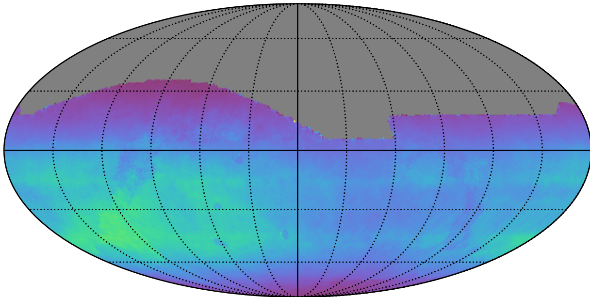
roll_pause_mjdp180_v3.4_10yrs All sky all bands: Normalized Teff
