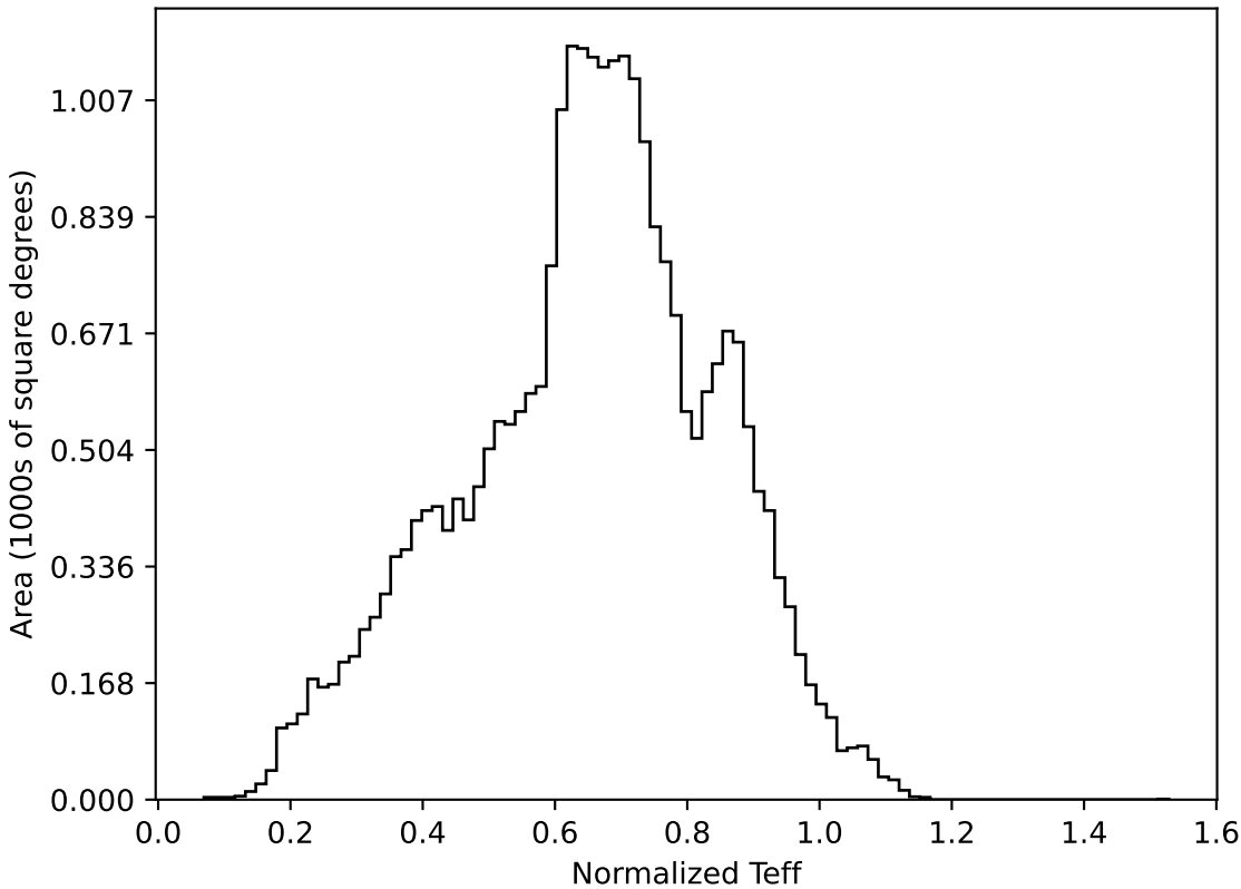
roll_pause_mjdp180_v3.4_10yrs All sky all bands: Normalized Teff
