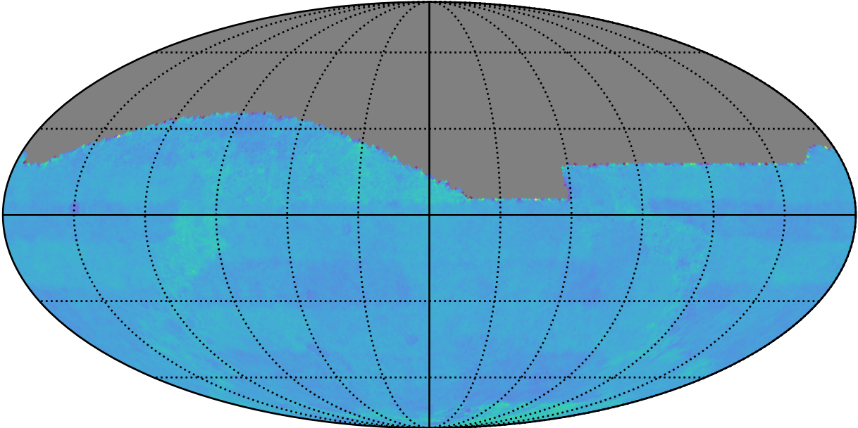
roll_pause_mjdp180_v3.4_10yrs All sky: Normalized Proper Motion Uncert @ 24.0
