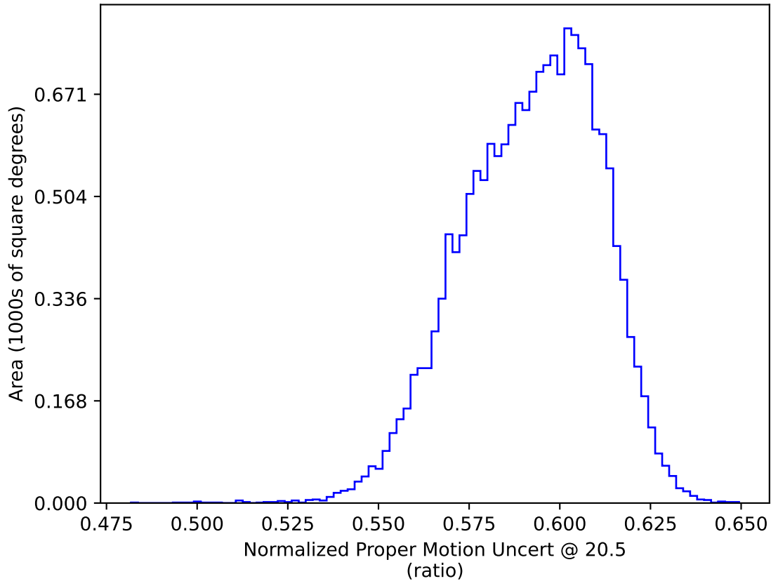
roll_pause_mjdp180_v3.4_10yrs WFD: Normalized Proper Motion Uncert @ 20.5
