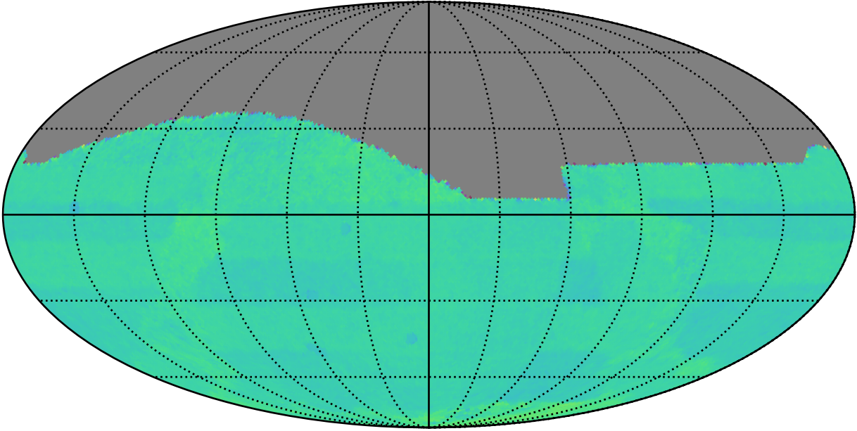
roll_pause_mjdp180_v3.4_10yrs All sky: Normalized Proper Motion Uncert @ 20.5
