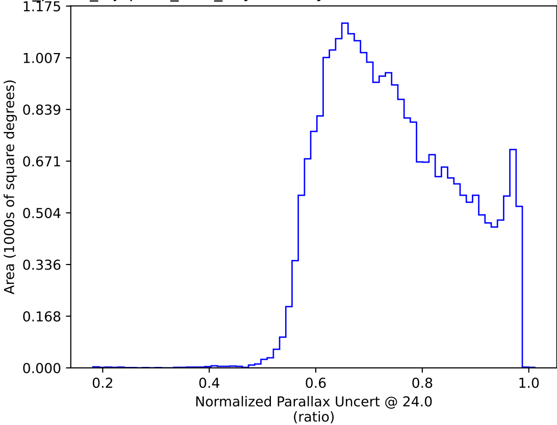
roll_pause_mjdp180_v3.4_10yrs All sky: Normalized Parallax Uncert @ 24.0
