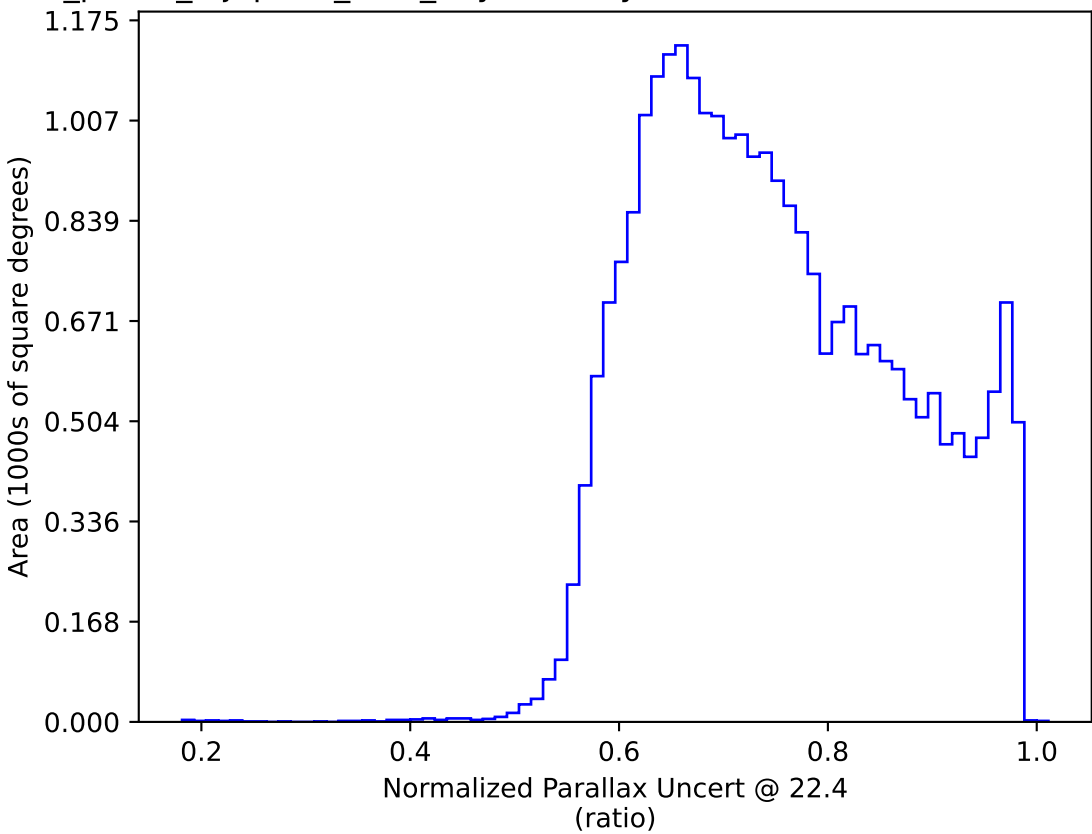
roll_pause_mjdp180_v3.4_10yrs All sky: Normalized Parallax Uncert @ 22.4
