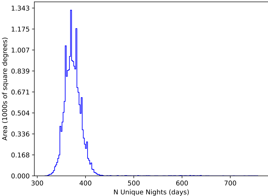
roll_pause_mjdp180_v3.4_10yrs WFD all bands: N Unique Nights
