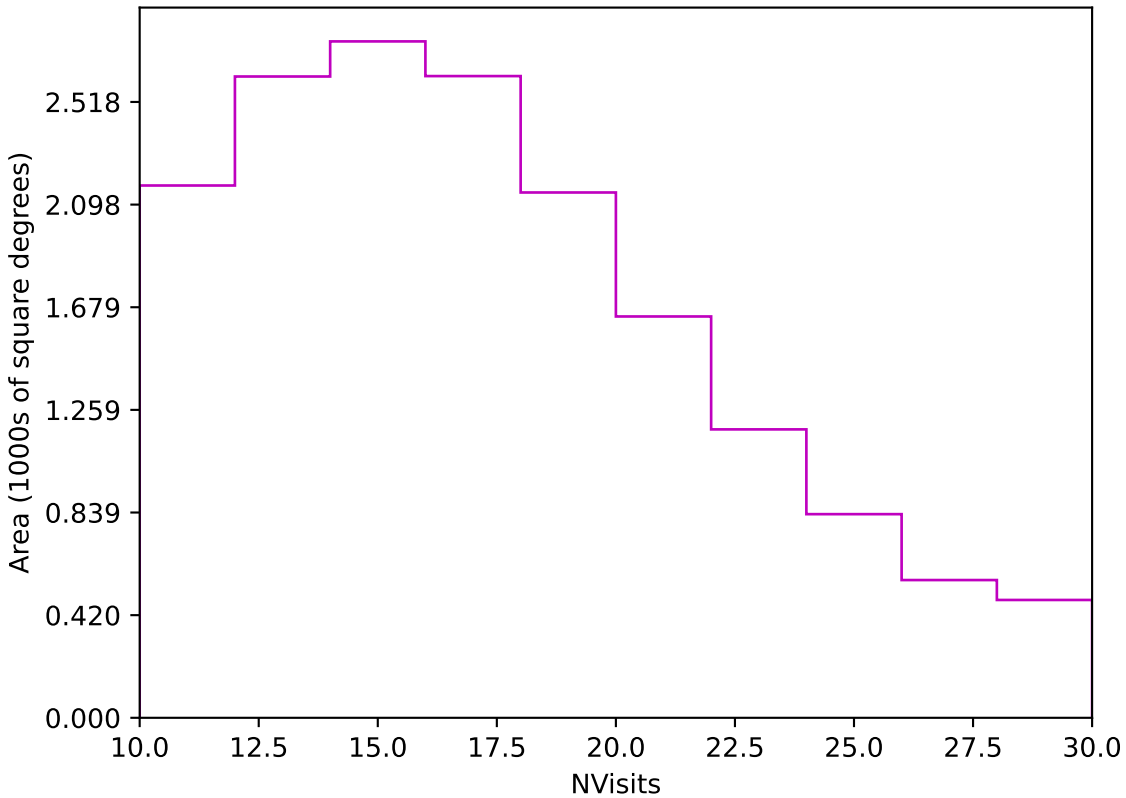
roll_pause_mjdp180_v3.4_10yrs Yr 3-4 z band: NVisits
