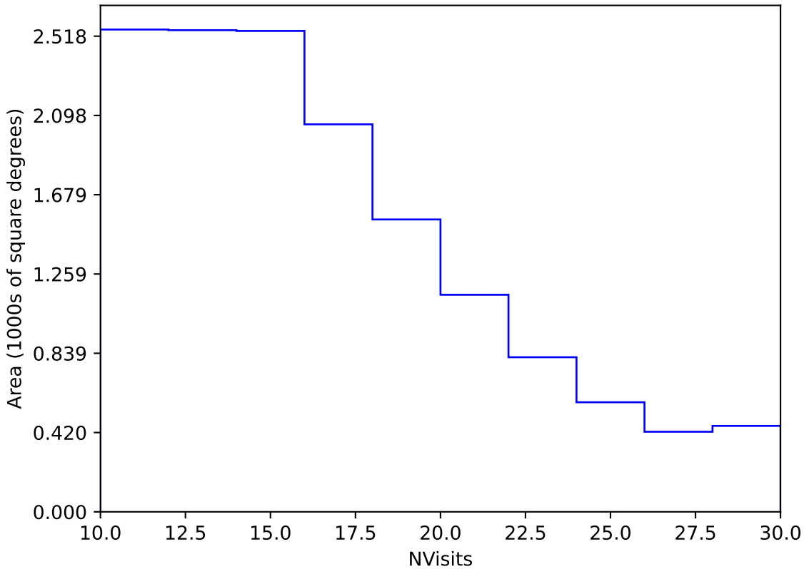
roll_pause_mjdp180_v3.4_10yrs Yr 3-4 y band: NVisits
