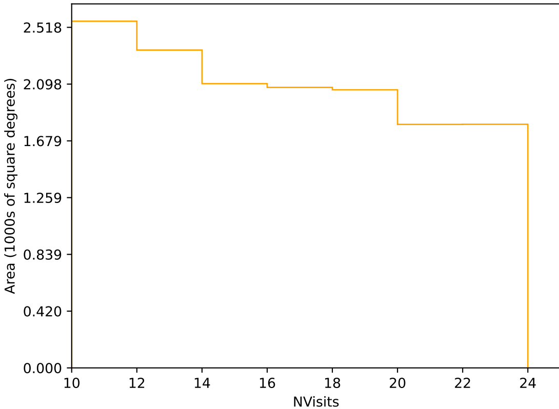
roll_pause_mjdp180_v3.4_10yrs Yr 3-4 r band: NVisits
