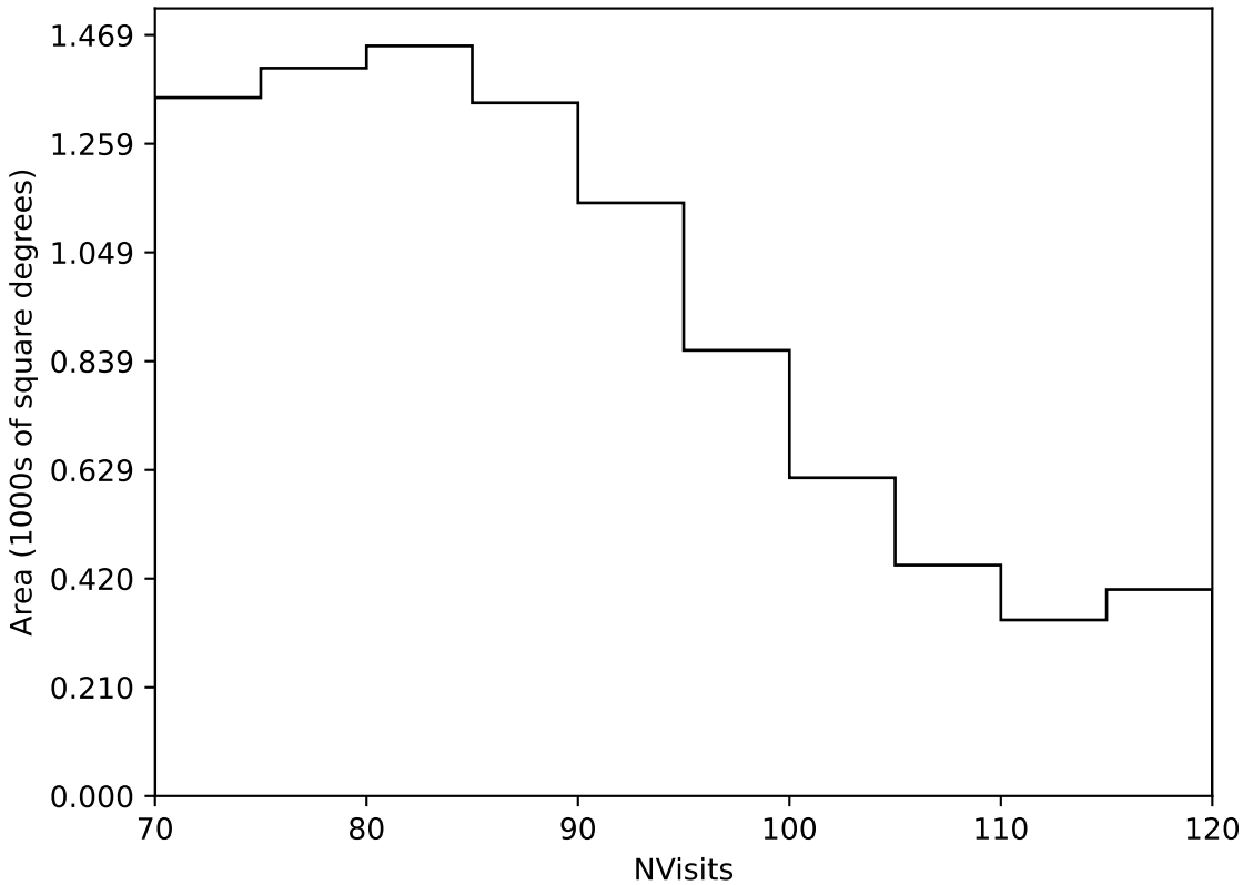
roll_pause_mjdp180_v3.4_10yrs Yr 3-4 all bands: NVisits
