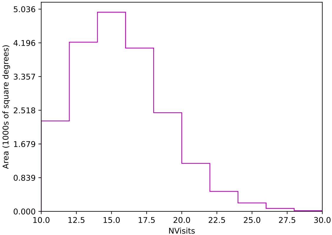
roll_pause_mjdp180_v3.4_10yrs Yr 1 z band: NVisits
