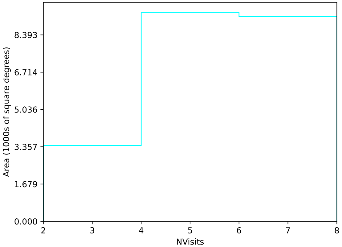
roll_pause_mjdp180_v3.4_10yrs Yr 1 u band: NVisits
