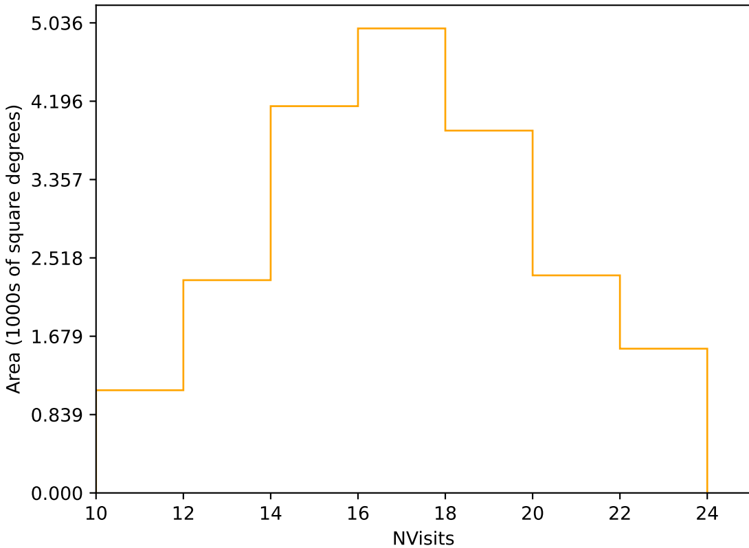
roll_pause_mjdp180_v3.4_10yrs Yr 1 r band: NVisits
