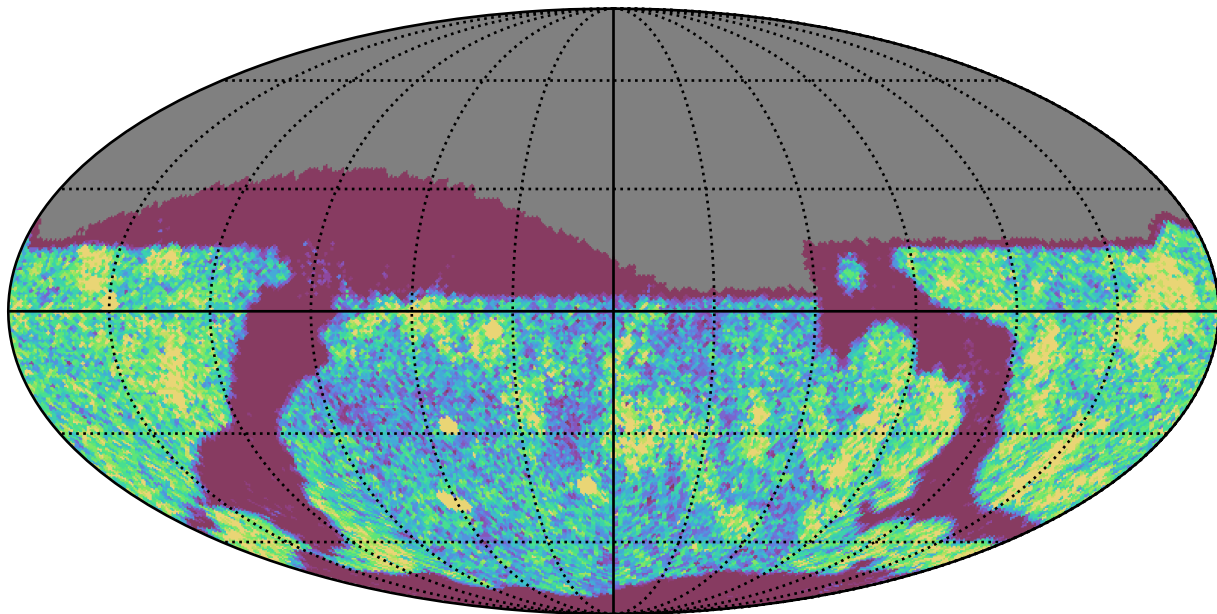
roll_pause_mjdp180_v3.4_10yrs Yr 1 i band: NVisits
