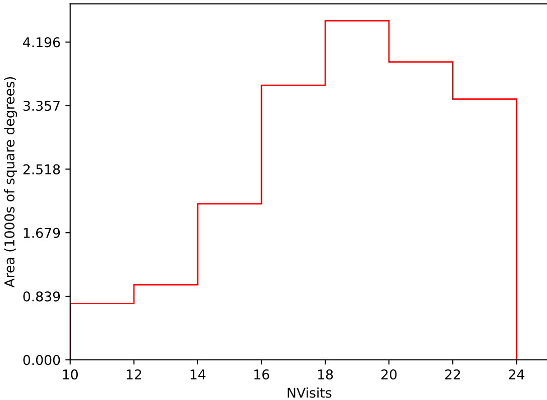
roll_pause_mjdp180_v3.4_10yrs Yr 1 i band: NVisits
