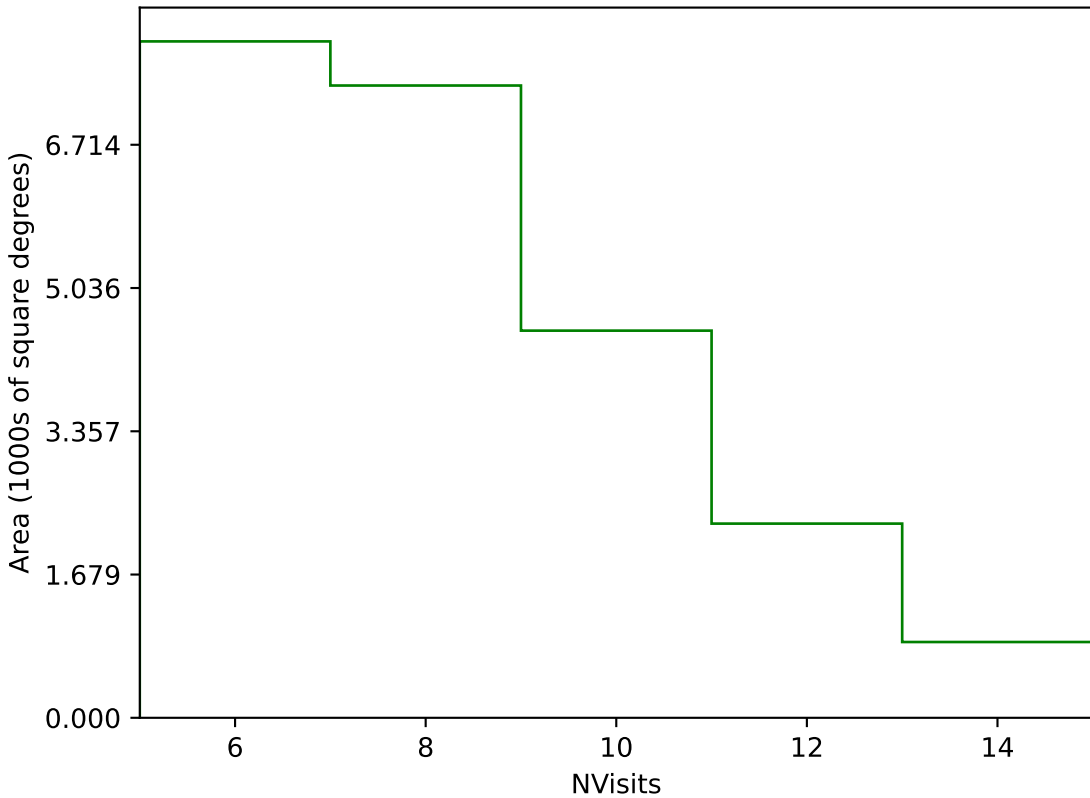
roll_pause_mjdp180_v3.4_10yrs Yr 1 g band: NVisits
