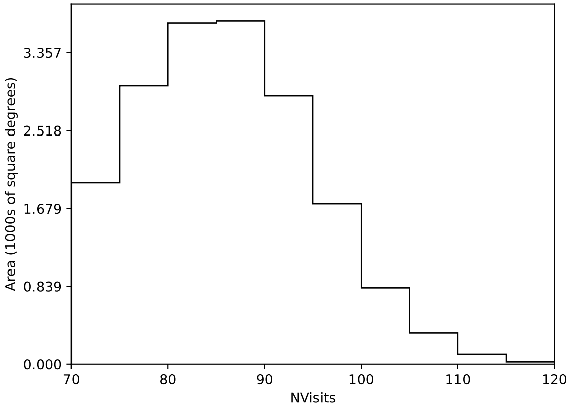
roll_pause_mjdp180_v3.4_10yrs Yr 1 all bands: NVisits
