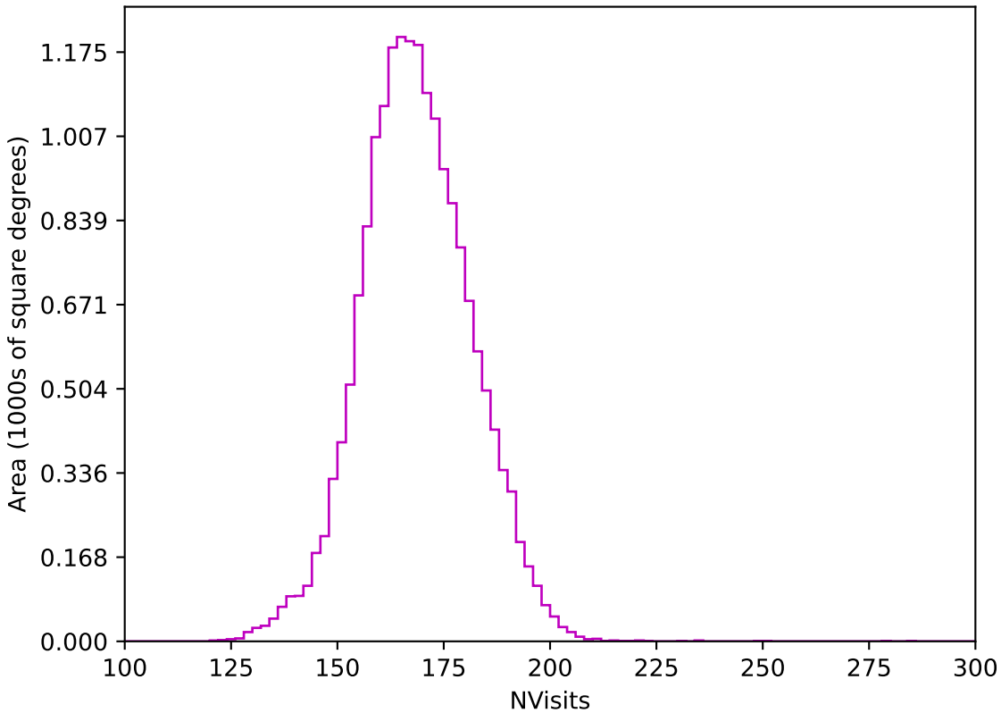
roll_pause_mjdp180_v3.4_10yrs WFD z band: NVisits
