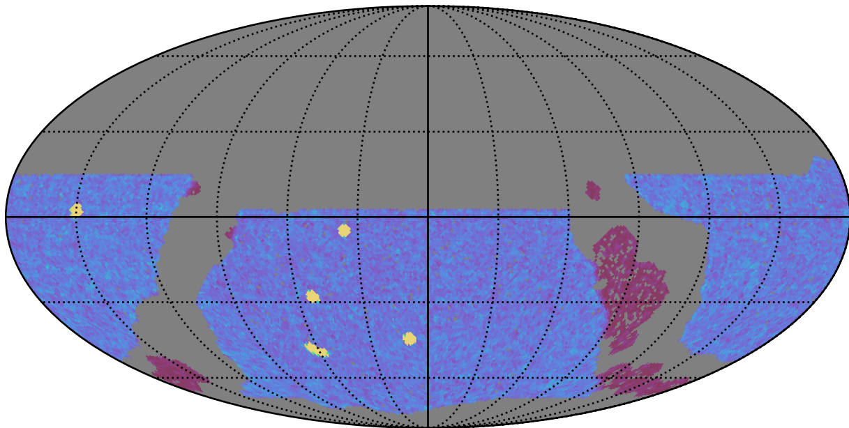
roll_pause_mjdp180_v3.4_10yrs WFD y band: NVisits
