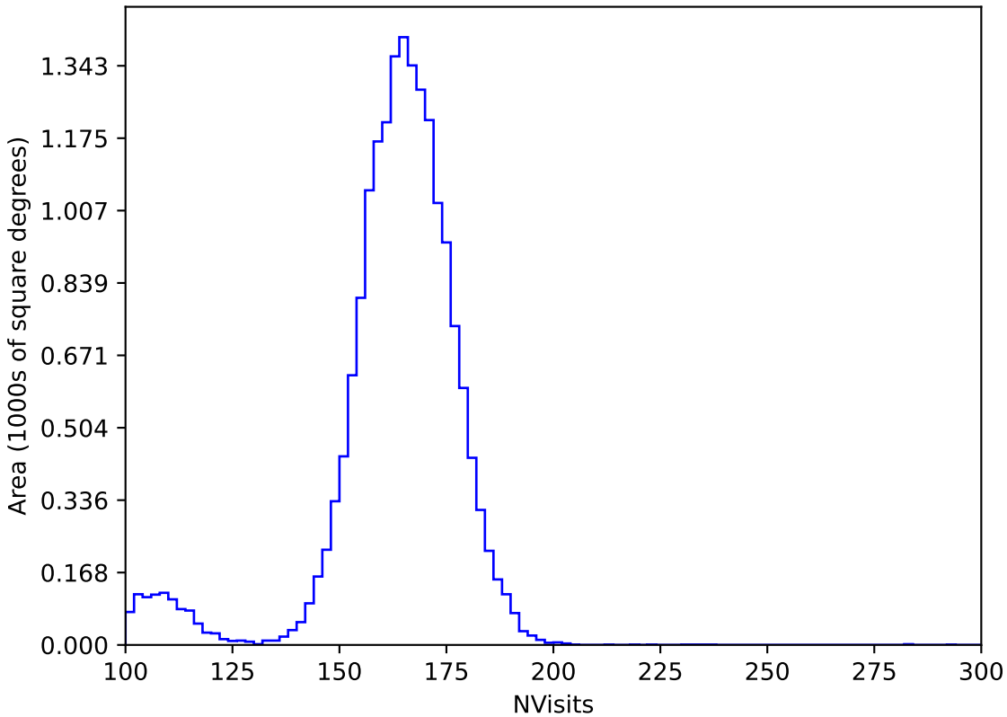
roll_pause_mjdp180_v3.4_10yrs WFD y band: NVisits
