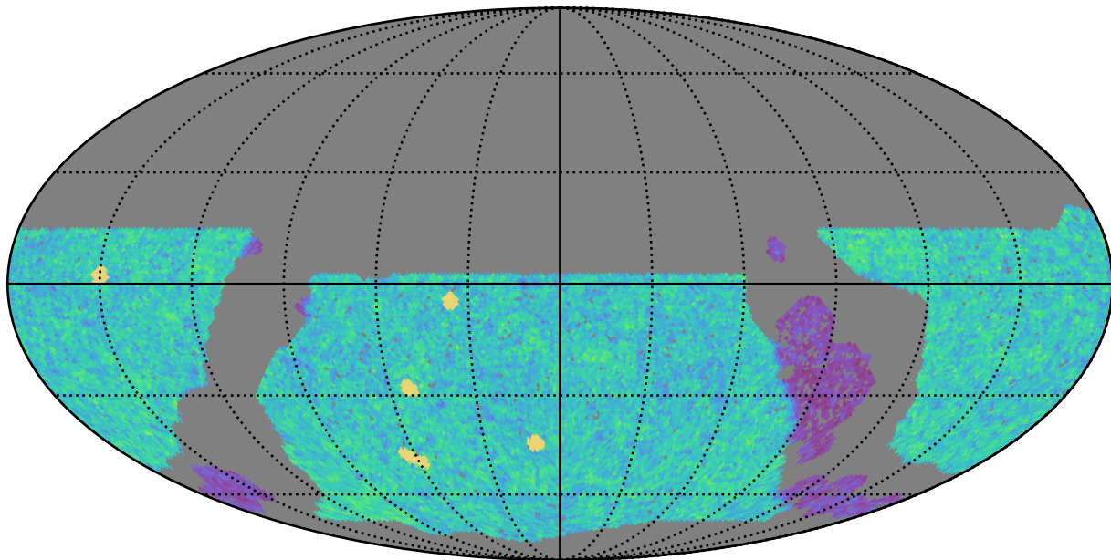
roll_pause_mjdp180_v3.4_10yrs WFD u band: NVisits
