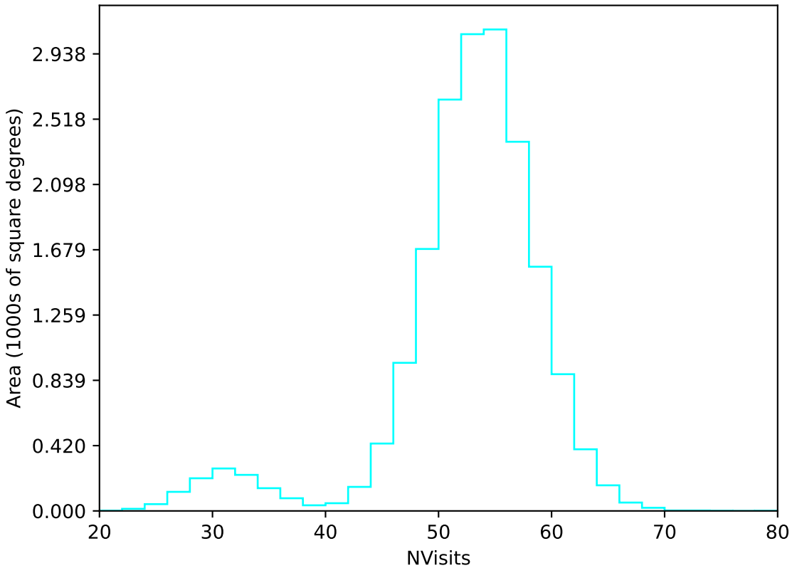
roll_pause_mjdp180_v3.4_10yrs WFD u band: NVisits
