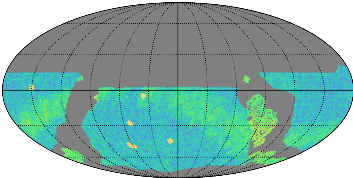
roll_pause_mjdp180_v3.4_10yrs WFD r band: NVisits
