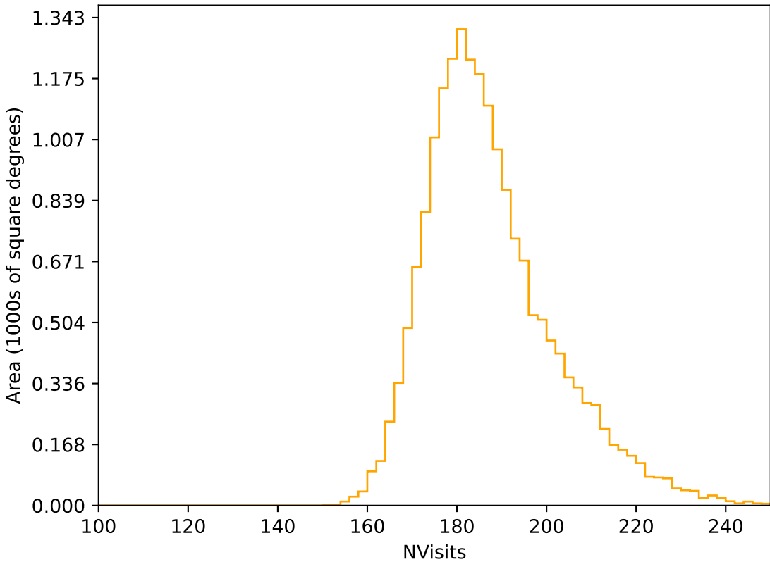
roll_pause_mjdp180_v3.4_10yrs WFD r band: NVisits
