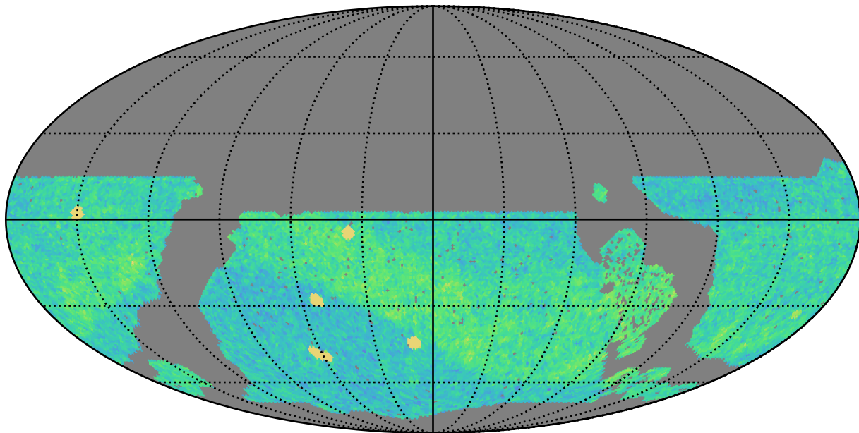
roll_pause_mjdp180_v3.4_10yrs WFD i band: NVisits
