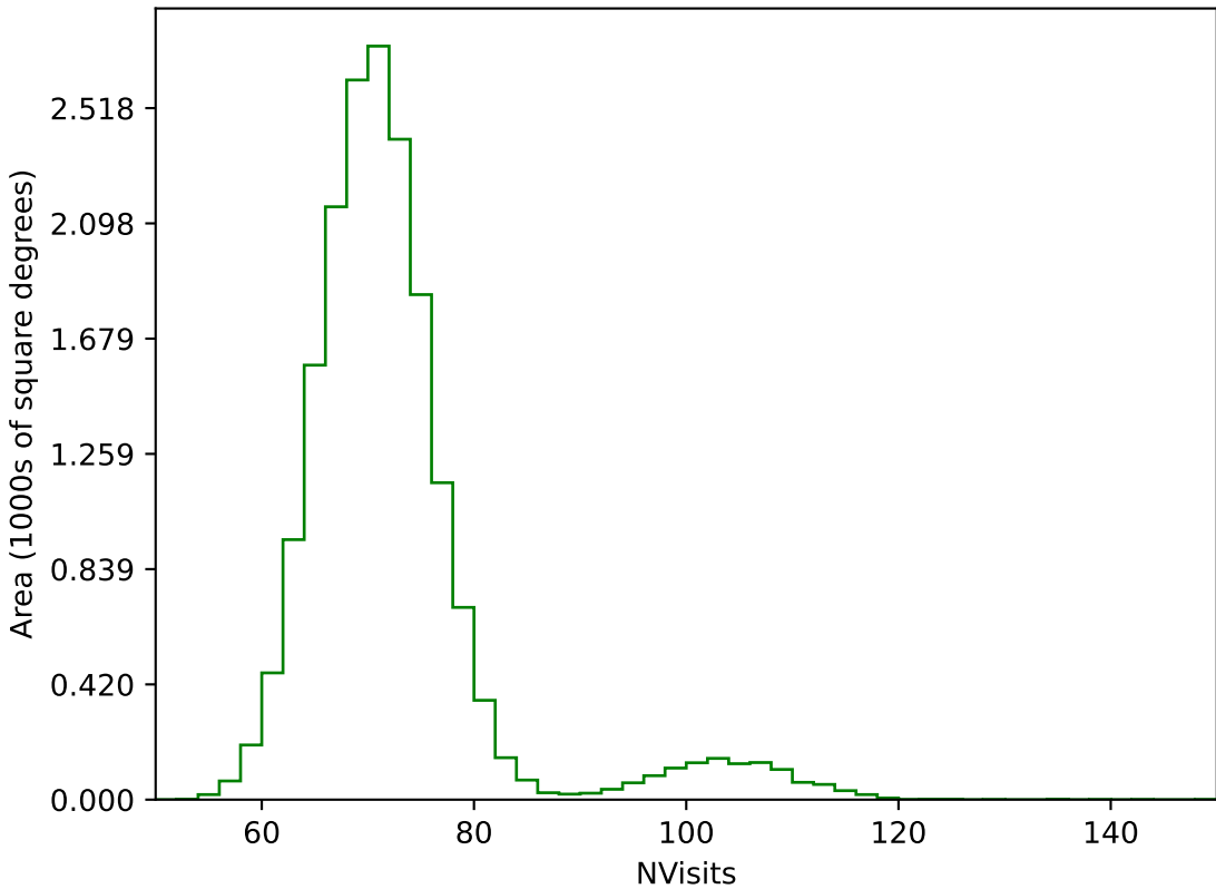
roll_pause_mjdp180_v3.4_10yrs WFD g band: NVisits
