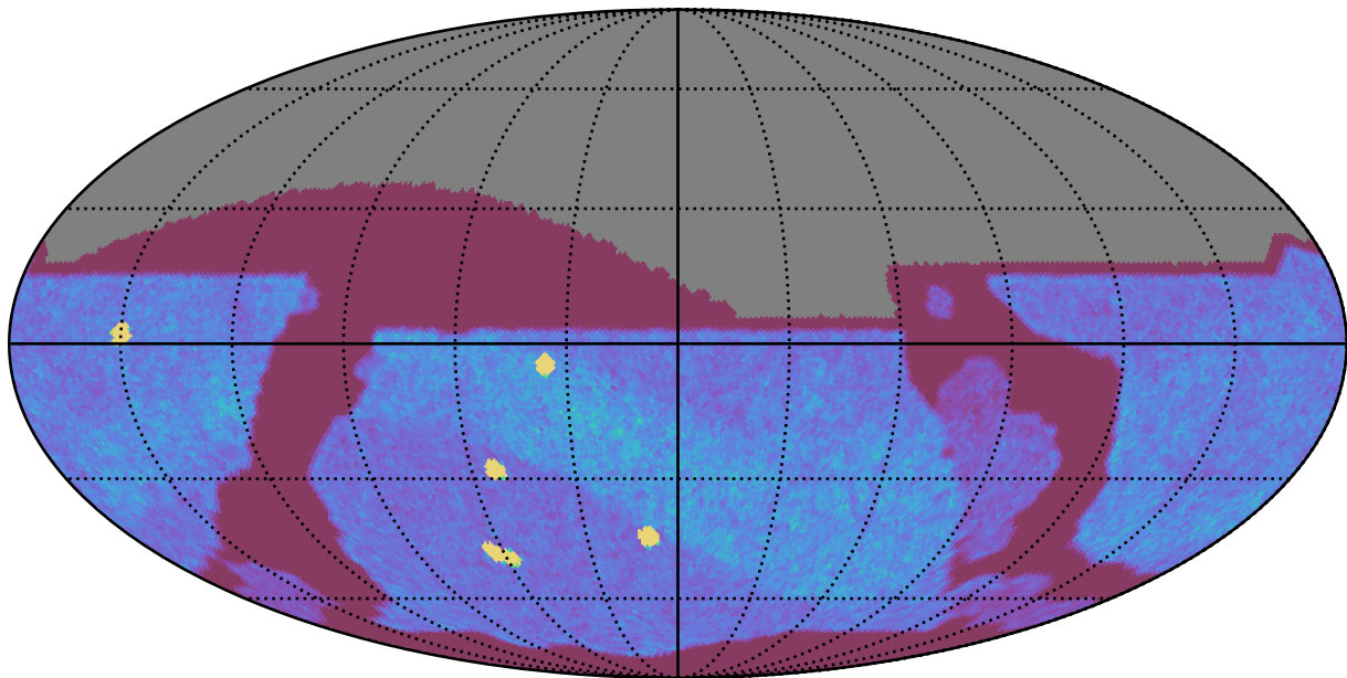
roll_pause_mjdp180_v3.4_10yrs All sky z band: NVisits
