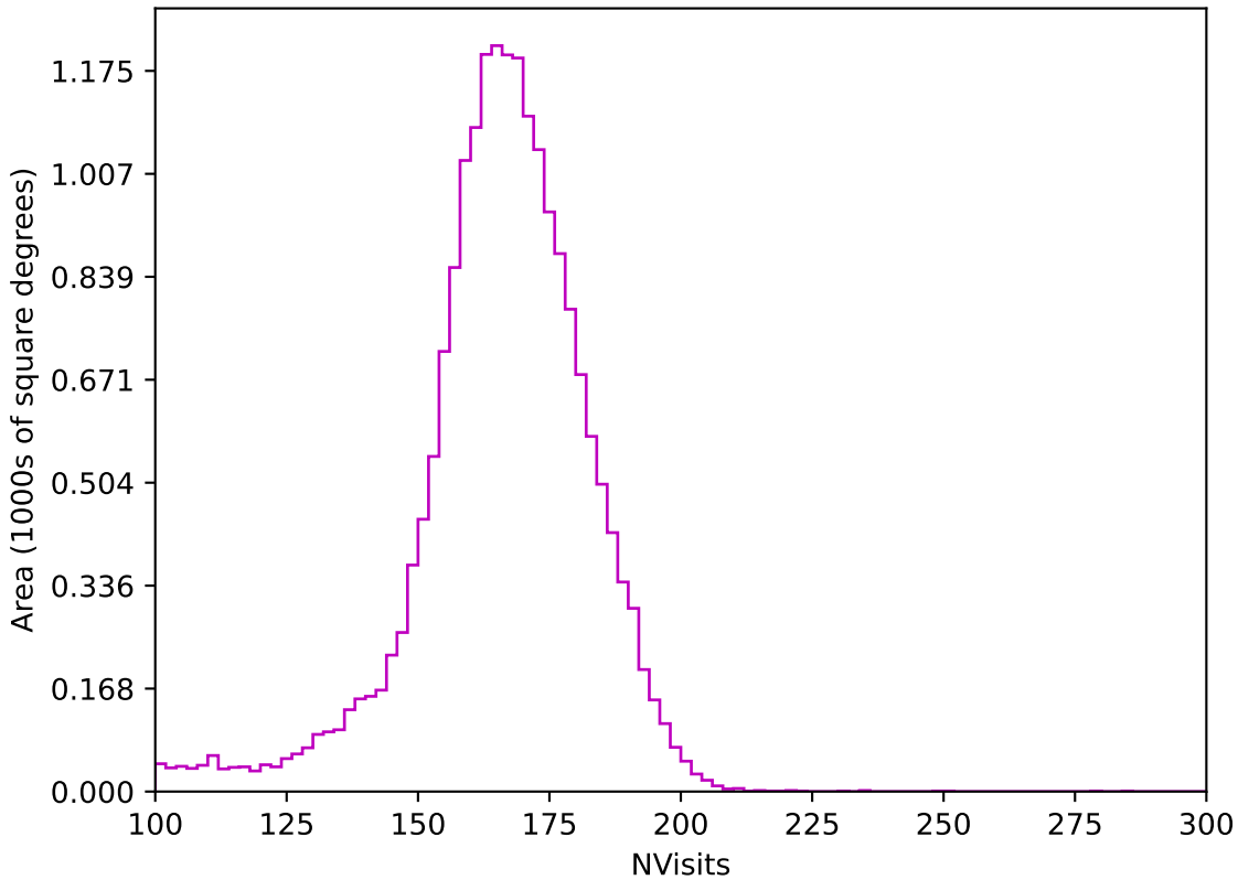
roll_pause_mjdp180_v3.4_10yrs All sky z band: NVisits
