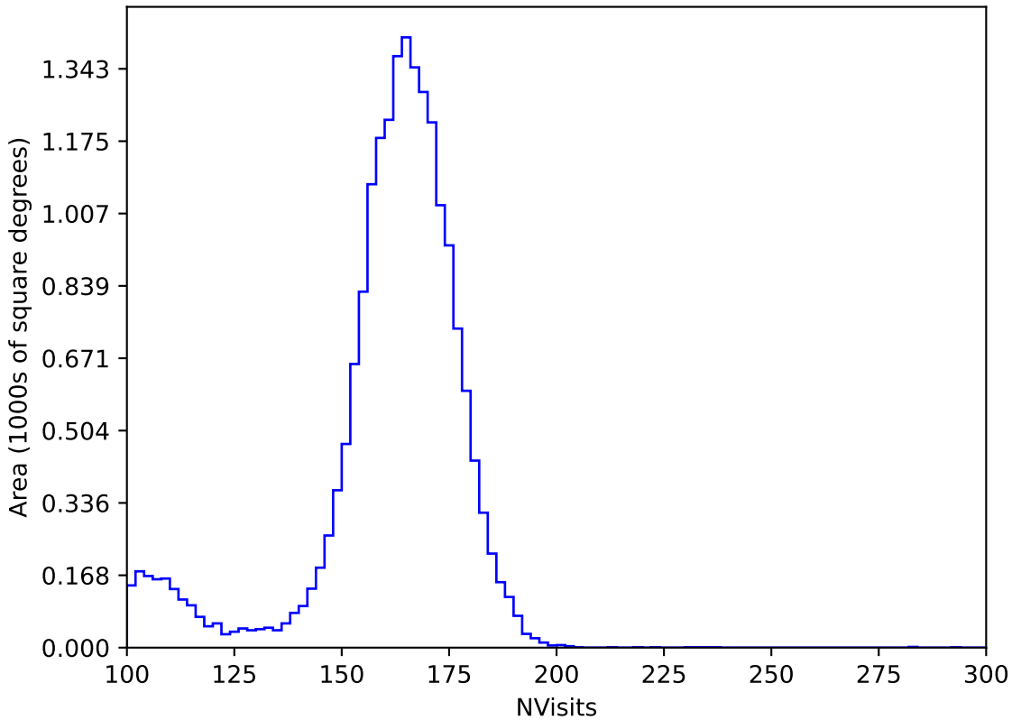
roll_pause_mjdp180_v3.4_10yrs All sky y band: NVisits
