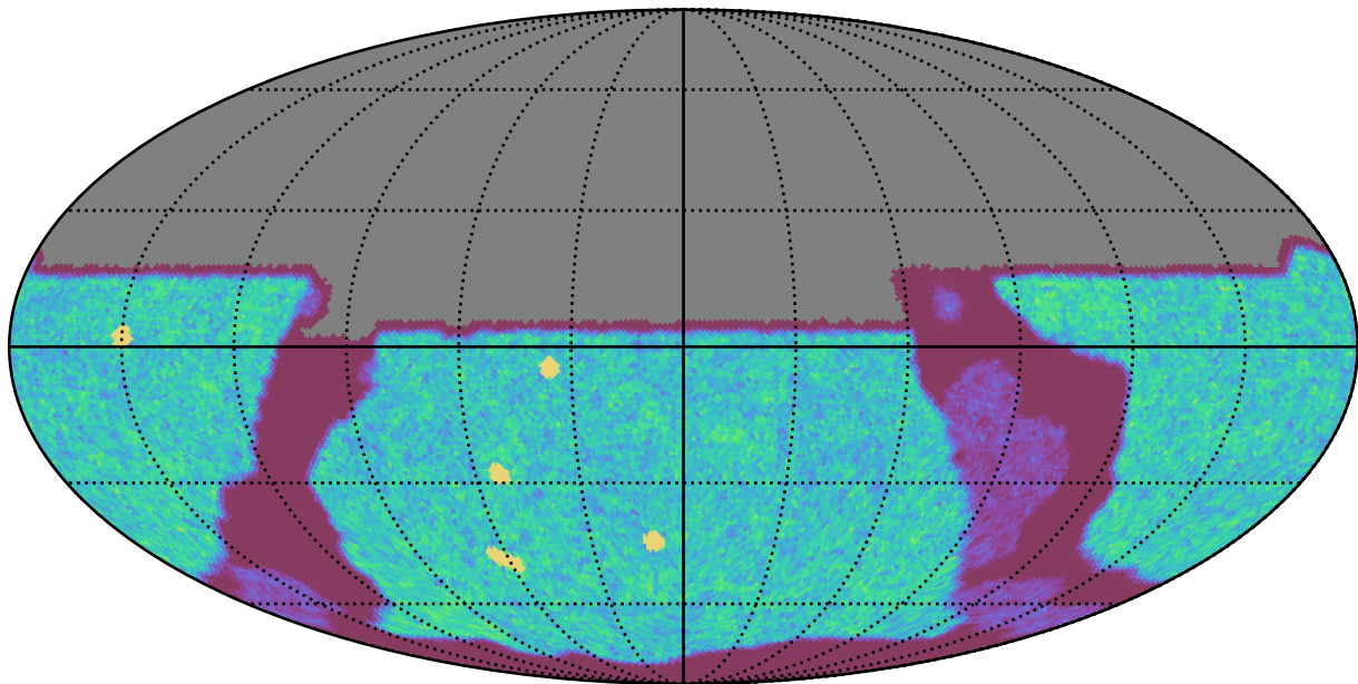
roll_pause_mjdp180_v3.4_10yrs All sky u band: NVisits
