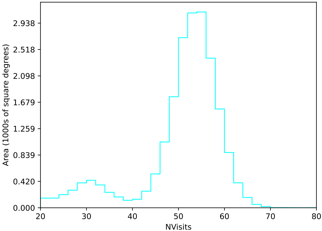
roll_pause_mjdp180_v3.4_10yrs All sky u band: NVisits
