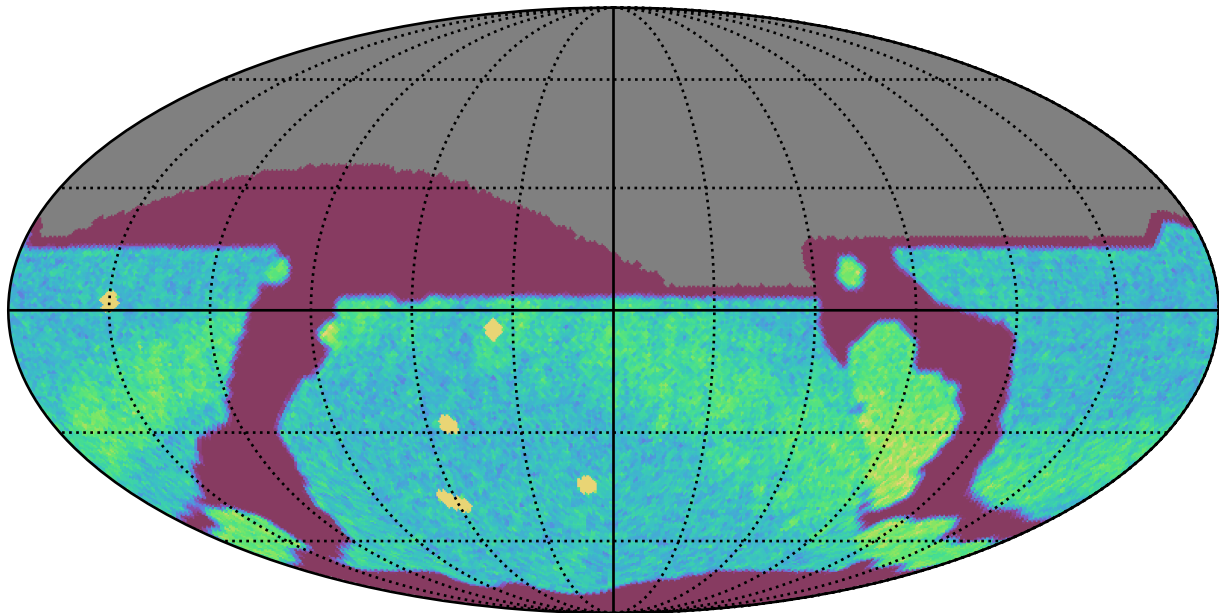
roll_pause_mjdp180_v3.4_10yrs All sky r band: NVisits
