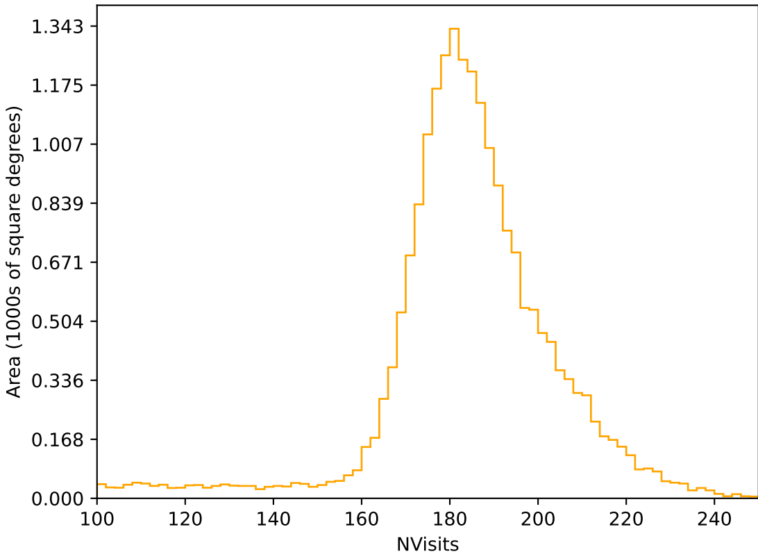
roll_pause_mjdp180_v3.4_10yrs All sky r band: NVisits
