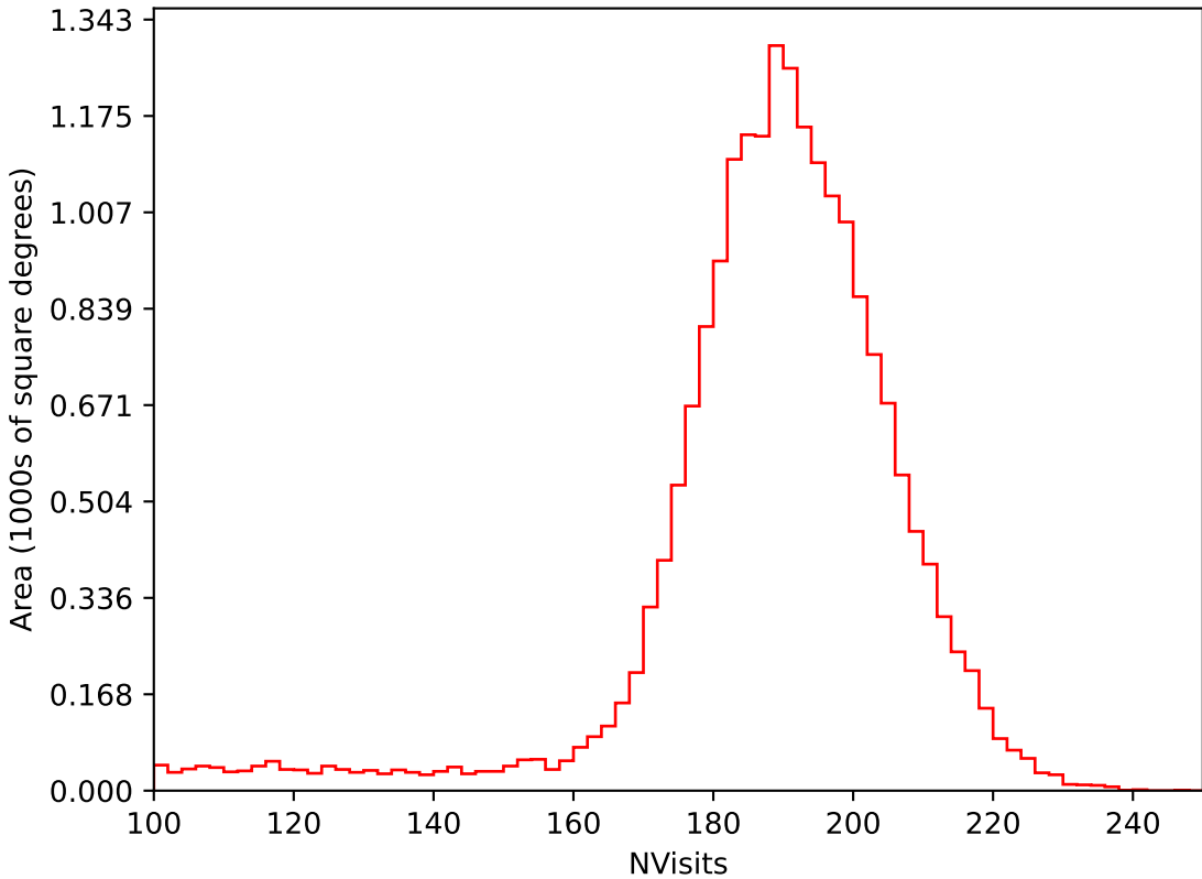
roll_pause_mjdp180_v3.4_10yrs All sky i band: NVisits
