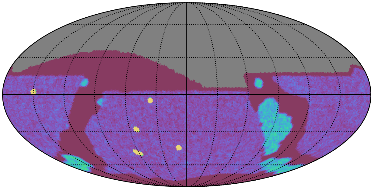
roll_pause_mjdp180_v3.4_10yrs All sky g band: NVisits
