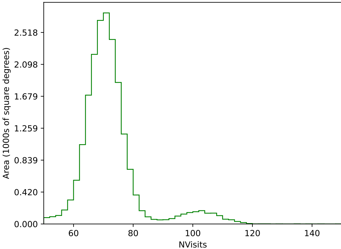
roll_pause_mjdp180_v3.4_10yrs All sky g band: NVisits
